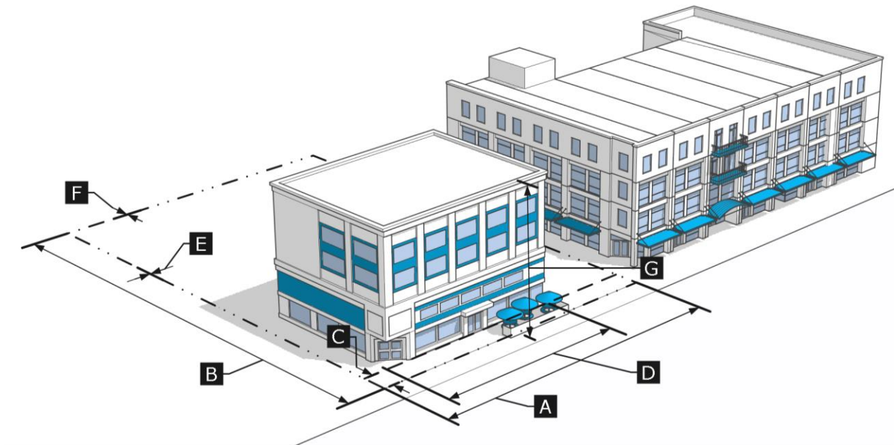
Figure 3-5: M-2 Dimensional Standards
