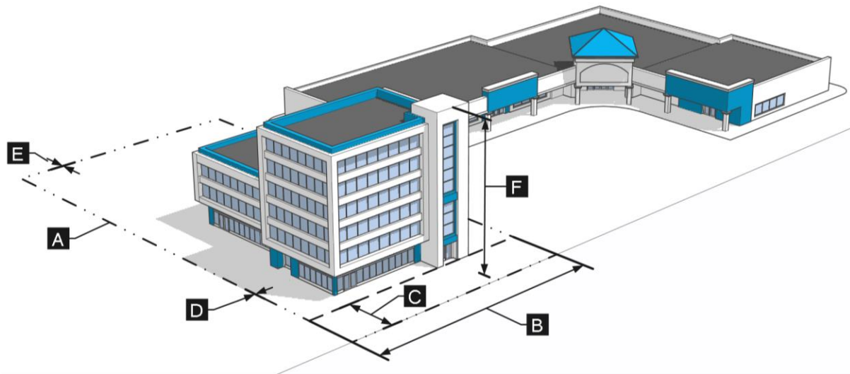
Figure 3-9: CG Dimensional Standards
