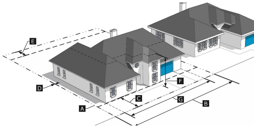
Figure 3-2: R-2 Dimensional Standards
