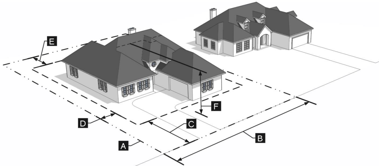
Figure 3-1: R-1 Dimensional Standards
