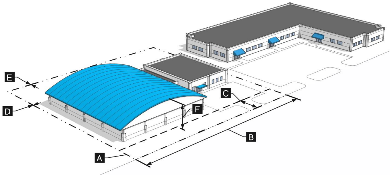
Figure 3-11: AA Dimensional Standards
