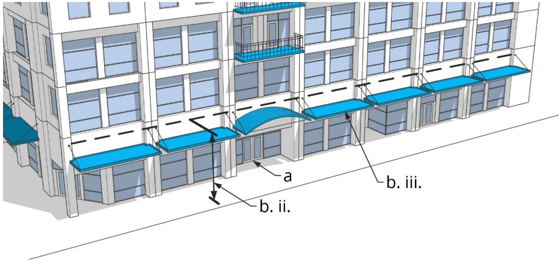
Figure 5-22: Nonresidential Uses at Grade
