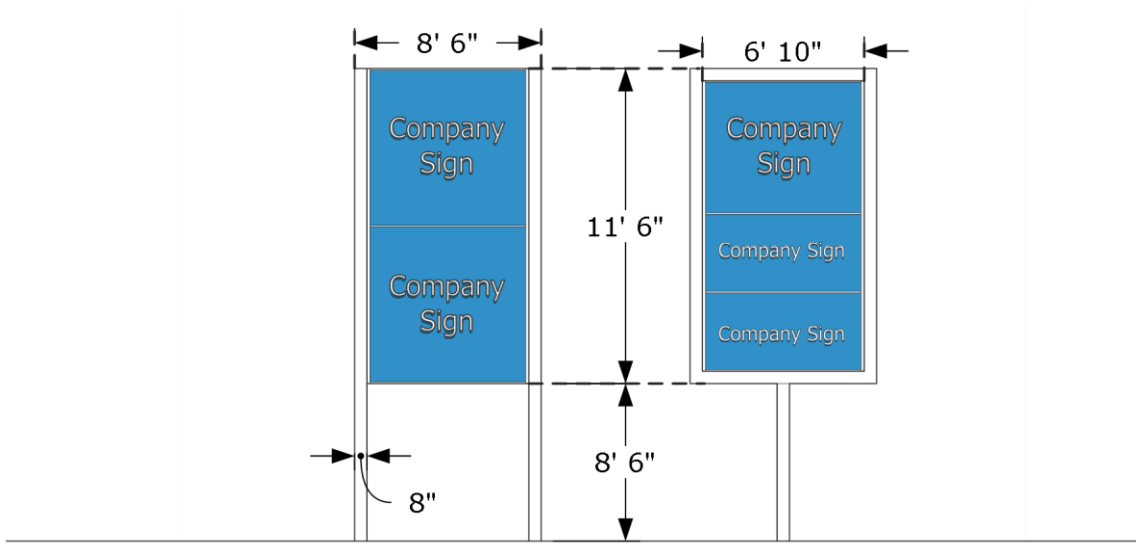
Figure 5-27: Pole Sign Supports
