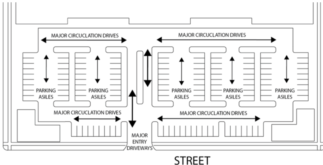
Figure 5-2: Vehicle Maneuvering
