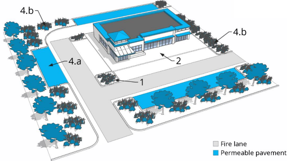
Figure 5-8: Parking Area Stormwater Drainage Standards
