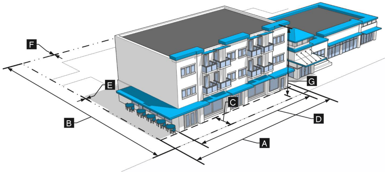
Figure 3-4: M-1 Dimensional Standards
