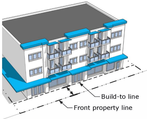
Figure 7-2: Build-to Line
