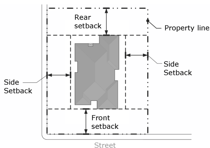
Figure 7-3: Setbacks
