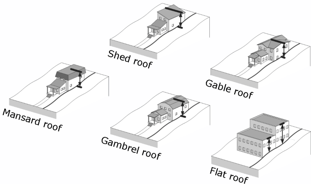
Figure 7-1: Building Height Measurement
