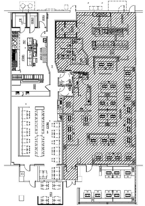
03 PHO BOWL FLOOR PLAN SCALE: NTS PHO BOWL INTERIOR : 2,400.1 S.F.
